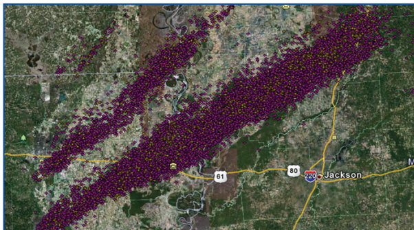
04.24.10 – Eastern Louisiana, US - ENTLN detects heavy lightning associated with a storm which generated an EF-4 tornado.
